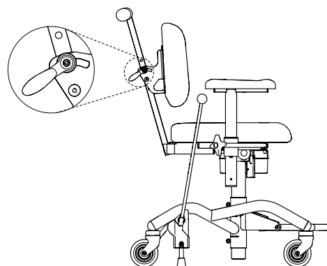
Figure 5.7. Fixed backrest mechanism with high back with push bar.
