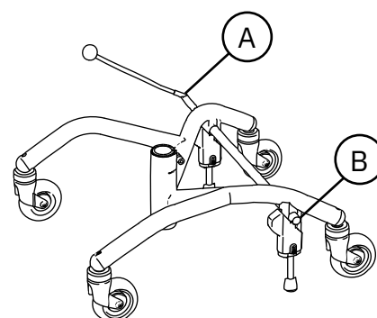
Figure 5.19. Brake lever.
