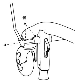
Figure 5.19. Brake lever.
