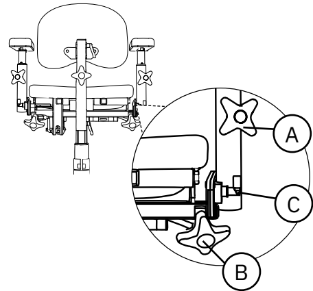
Figure 5.14. Foldable armrests.
