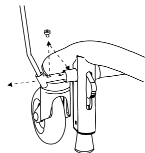
Figure 5.40. Brake lever.
