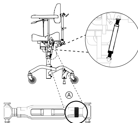
Figure 5.19. Crank handle for adjusting seat tilt.
