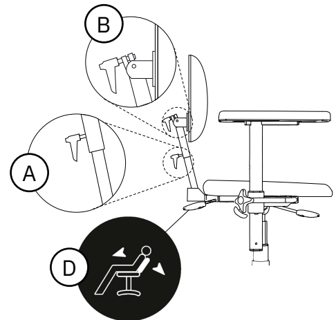
Figur 5.43. Ryggmekanism Comfort.
