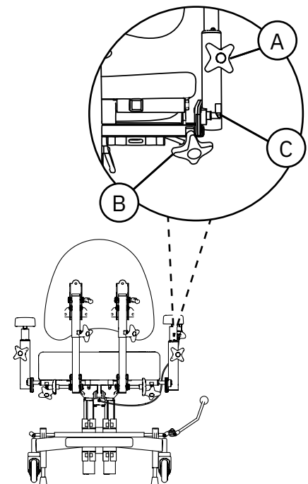
Figure 5.13. Foldable armrests.
