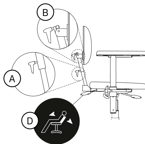
Figur 5.28. Ryggmekanism Comfort.
